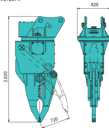
Multi-Demontagezange KVE720PR
