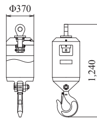
Ball Hook (For Wire rope dia. 30 mm) Weight: 450 kg
