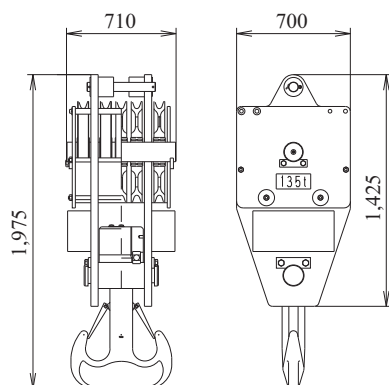
135 t Hook Weight: 1,700 kg
