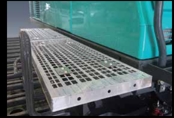
Removable walkway Walkways are provided on both the left and right sides of the base of the machine, allowing easier access for maintenance.
